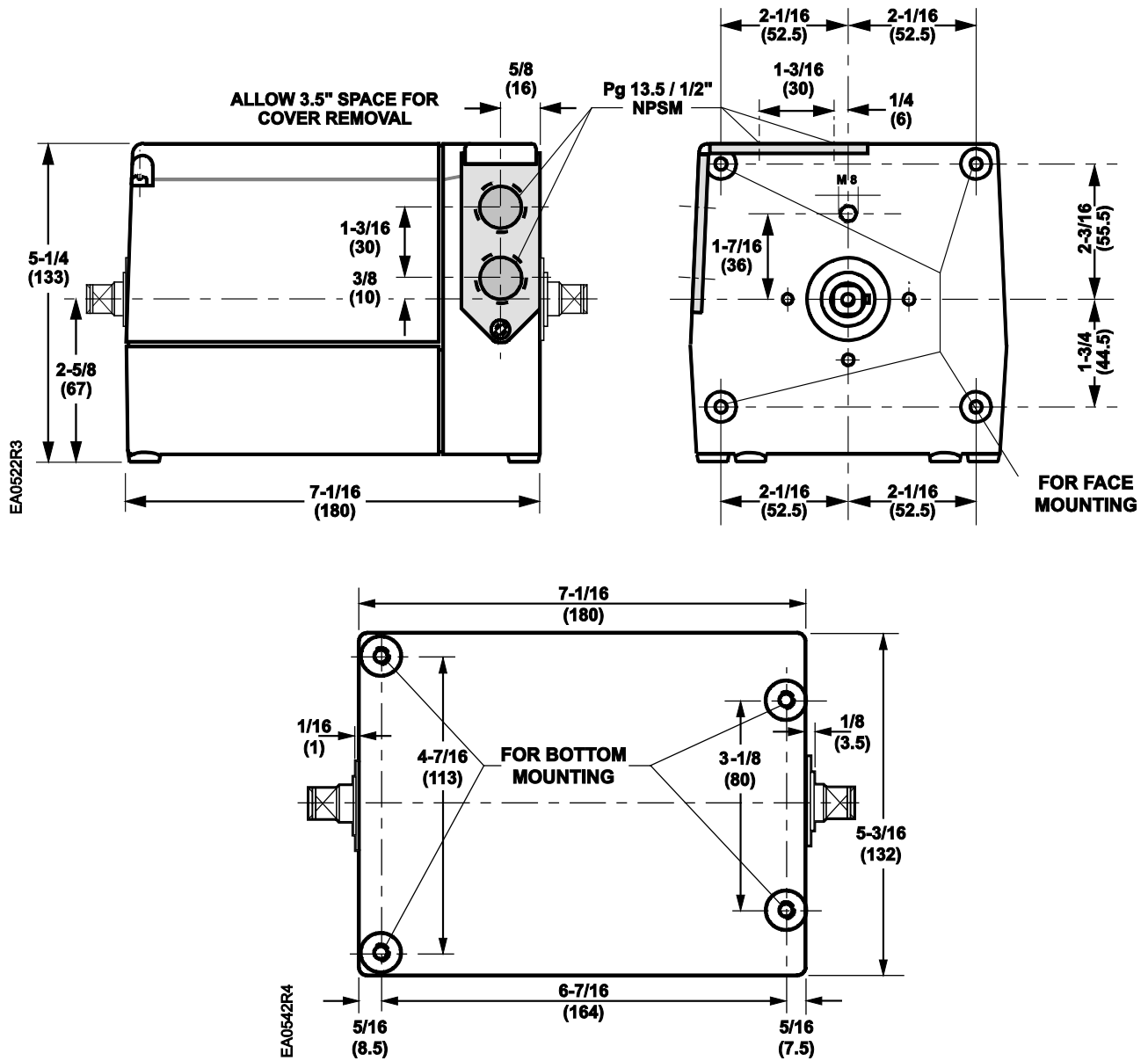
Figure 28. SQM5x.xxxRxx Dimensions.
